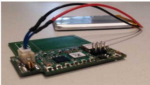
Figure 1 DUT Setup
