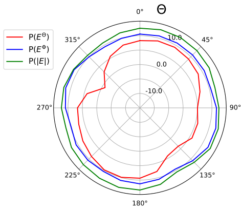
(c) xz-plane
