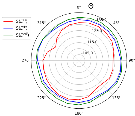
(c) xz-plane
