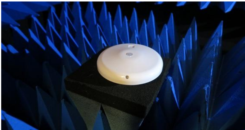
Figure 1 DUT Setup
