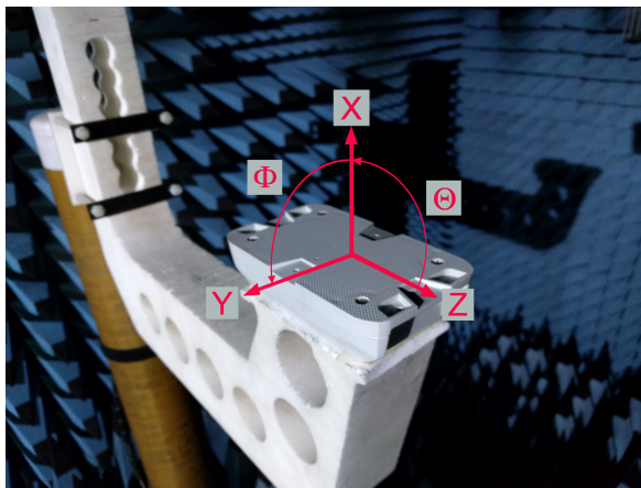
(a) Device under Test
