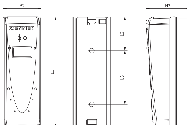
Dimensions split version
