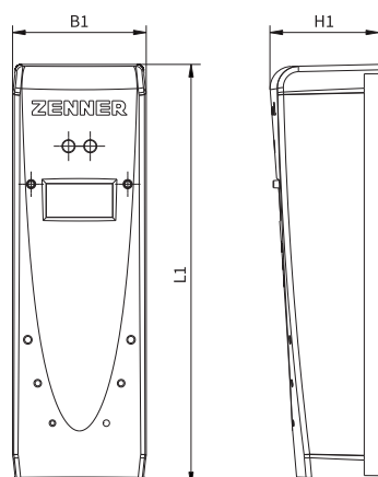
Dimensions compact version
