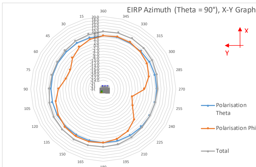
Fig. 12: 2D Pattern, X-Y plant at 863.1 MHz.
