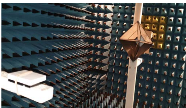
Fig. 1: Photo of test setup free space.
