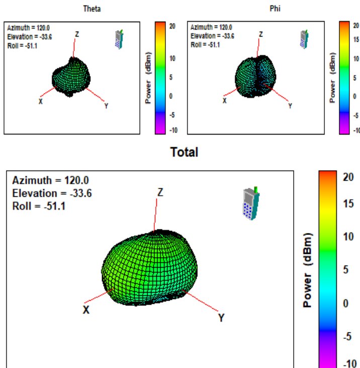
Fig. 15: 3D Pattern at 869.525 MHz.
