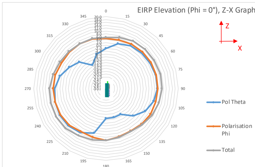
Fig. 17: 2D Pattern, Z-X plant at 869.525 MHz.
