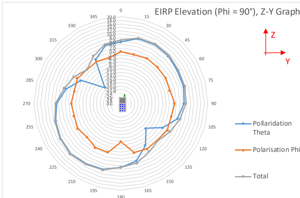
Fig. 14: 2D Pattern, Z-X plant at 863.1 MHz.
