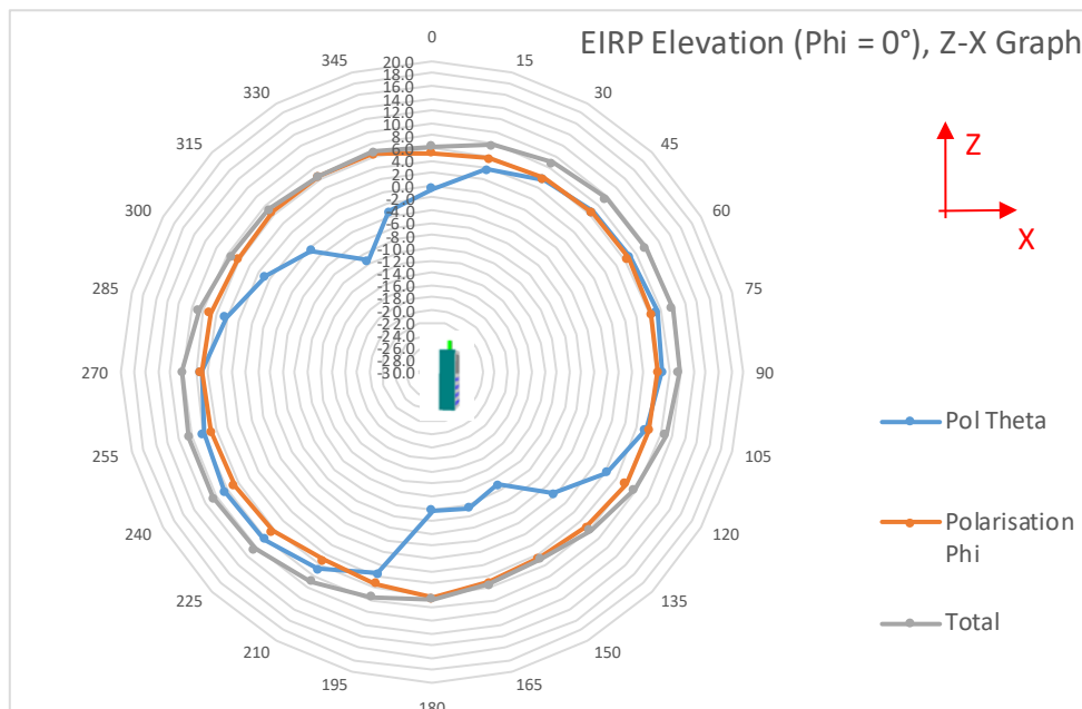
Fig. 9: 2D Pattern, Z-X plant at 865.1 MHz.
