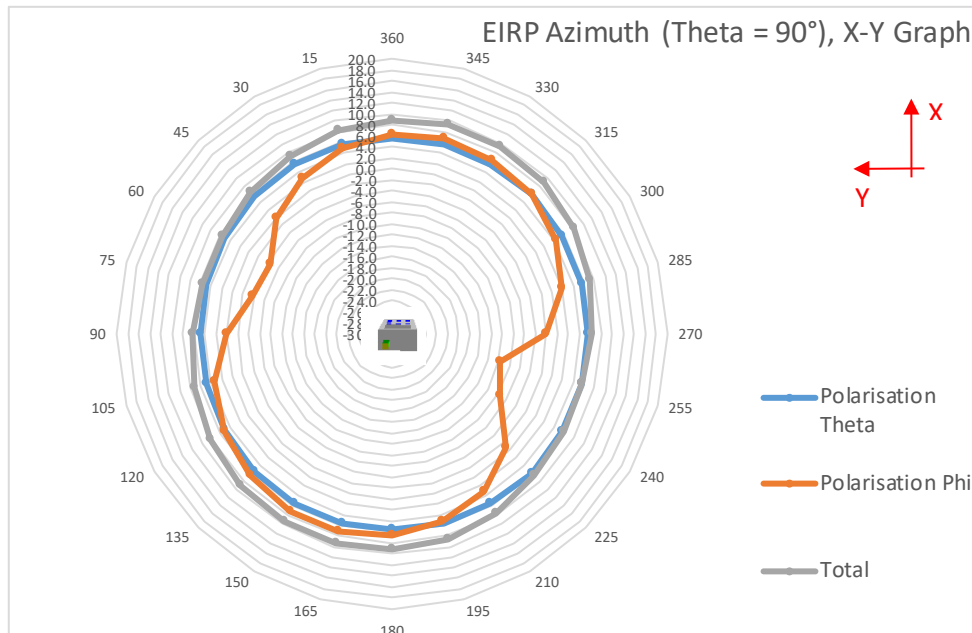
Fig. 16: 2D Pattern, X-Y plant at 869.525 MHz.
