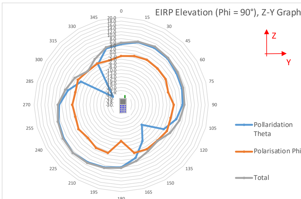
Fig. 18: 2D Pattern, Z-Y plant at 869.525 MHz.
