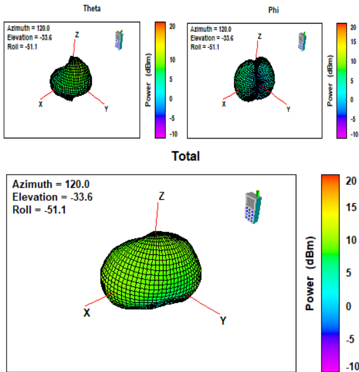
Fig. 7: 3D Pattern at 865.1 MHz.
