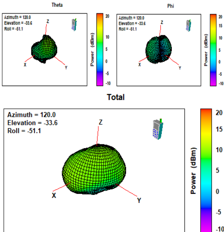
Fig. 11: 3D Pattern at 863.1 MHz.
