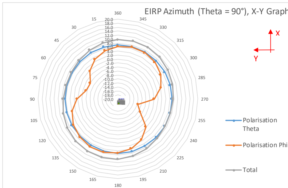
Fig. 8: 2D Pattern, X-Y plant at 865.1 MHz.
