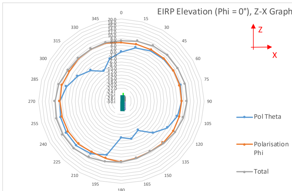
Fig. 13: 2D Pattern, Z-X plant at 863.1 MHz.
