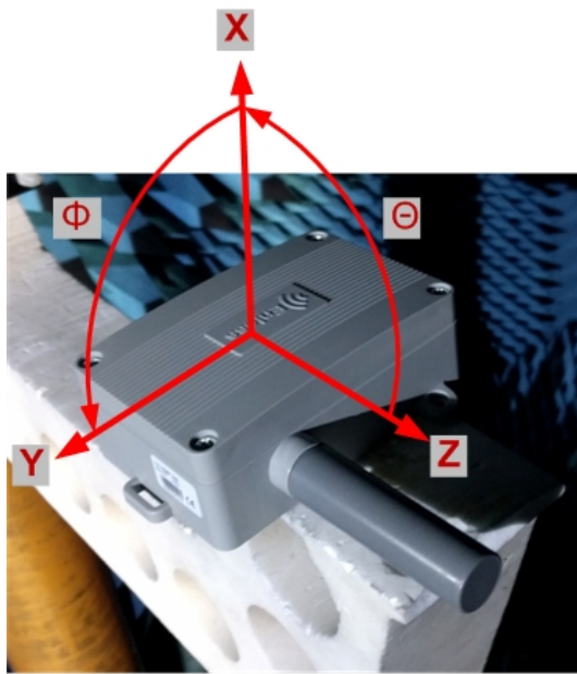
(a) Device under Test
