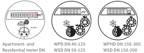
Fig. 1: ZENNER registers with modulator disc
