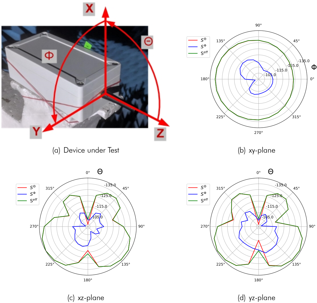
Figure 4.6: Rx Sensitivity Results for Channel: LOW-SF12BW125
