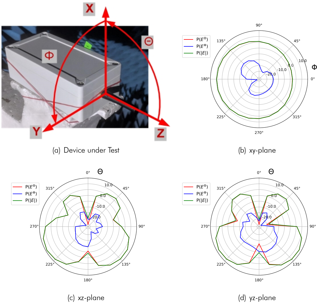
Figure 4.4: Tx Power Measurement Results for Channel: HIGH (RX2)
