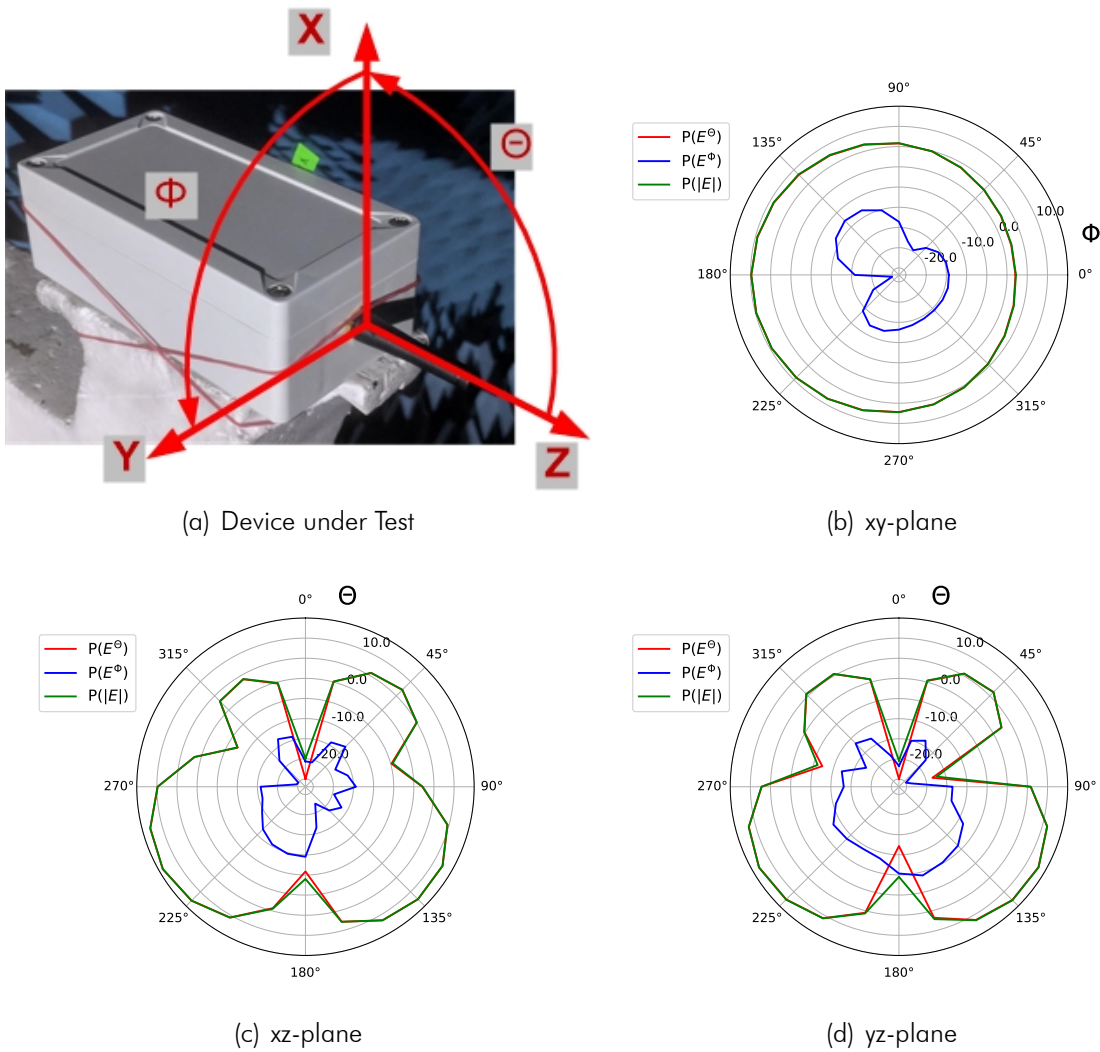
Figure 4.3: Tx Power Measurement Results for Channel: HIGH
