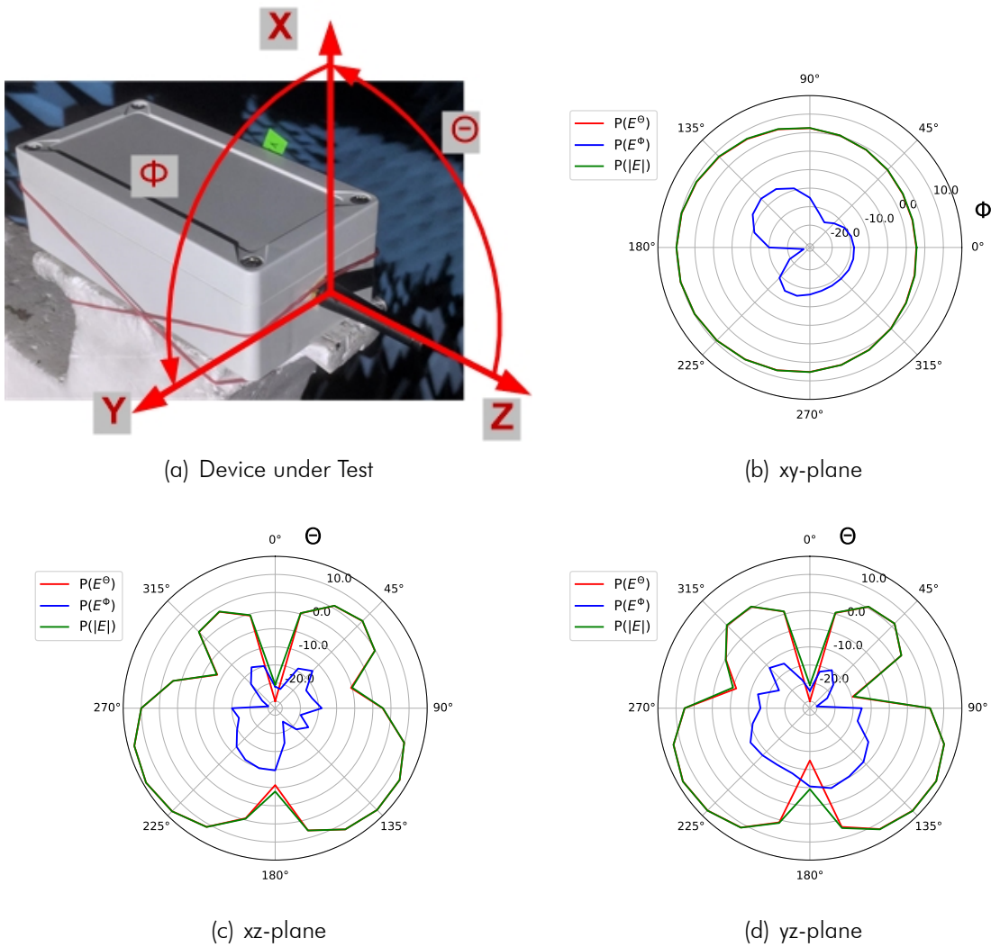
Figure 4.2: Tx Power Measurement Results for Channel: MID
