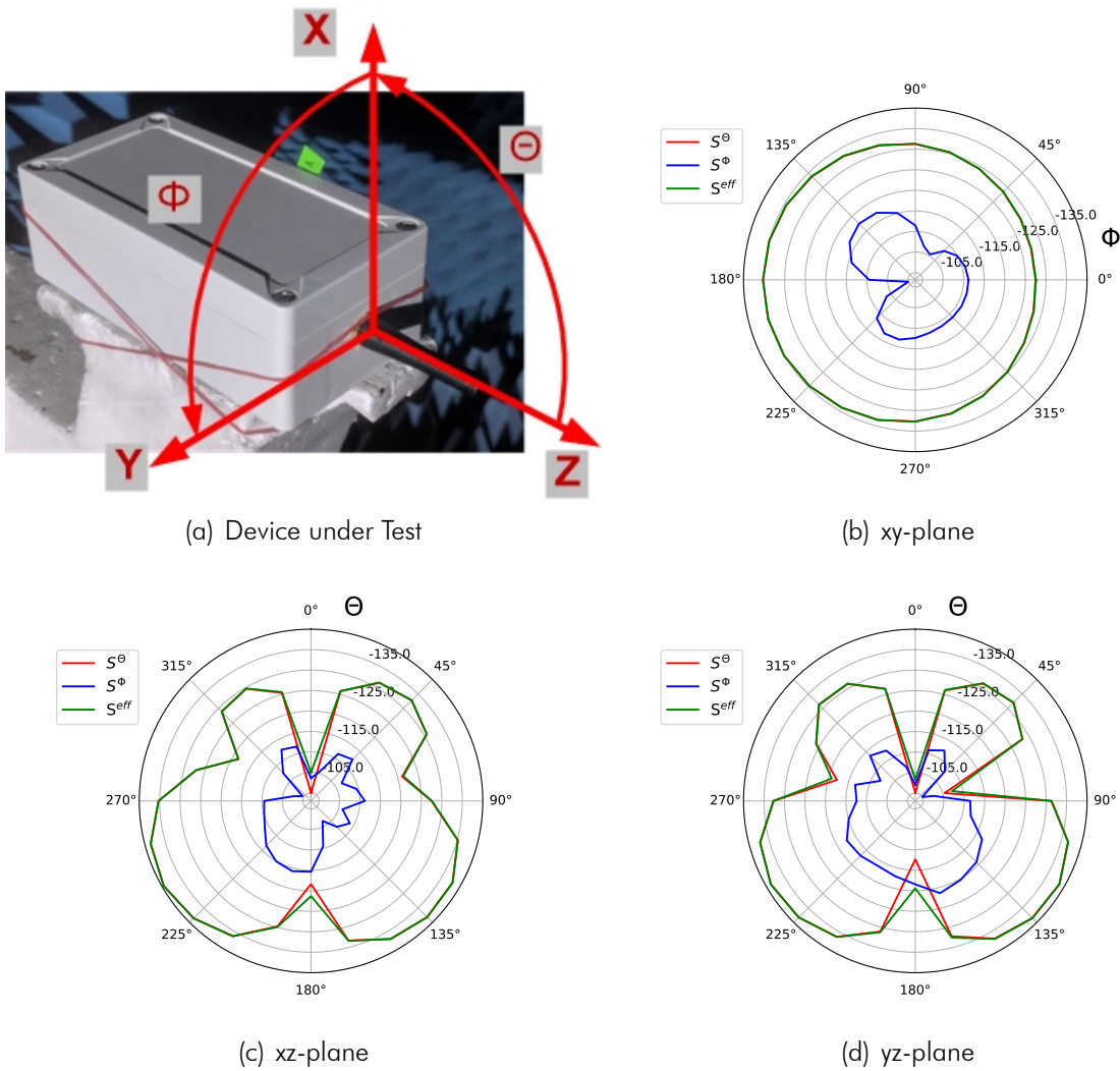
Figure 4.12: Rx Sensitivity Results for Channel: HIGH (RX2)-SF12BW125
