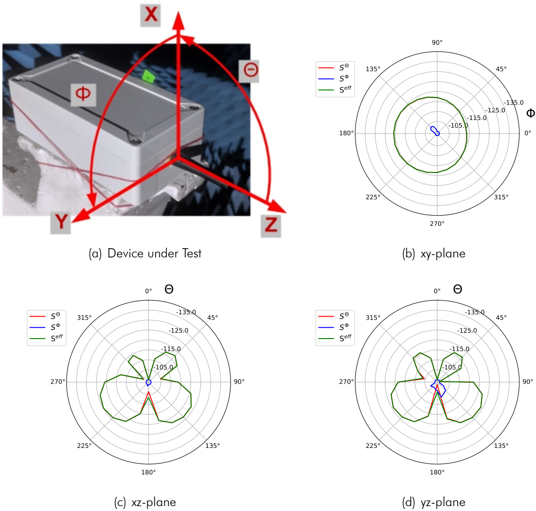
Figure 4.5: Rx Sensitivity Results for Channel: LOW-SF7BW125
