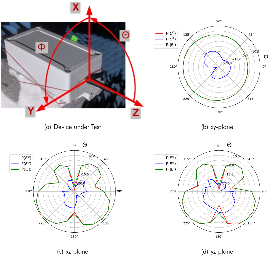
Figure 4.1: Tx Power Measurement Results for Channel: LOW
