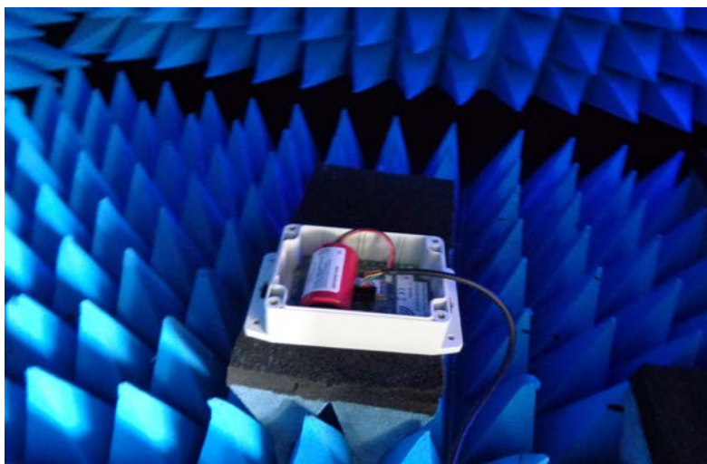
Figure 1 DUT Setup
