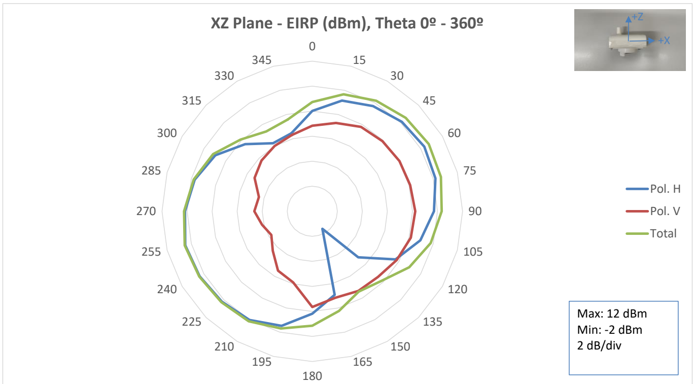
Fig. 11. XZ Plane EIRP, Free Space, 868.3 MHz.
