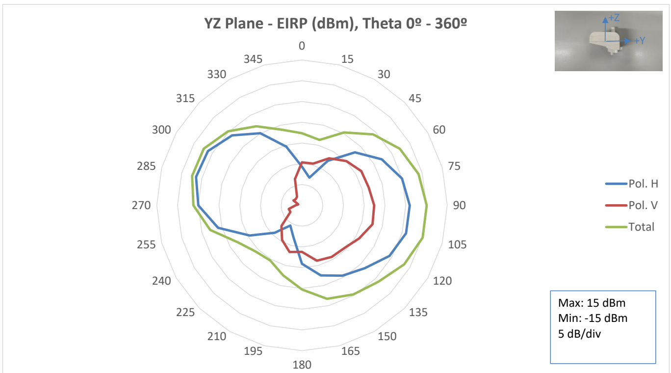
Fig. 9. YZ Plane EIRP, Free Space, 865.1 MHz.
