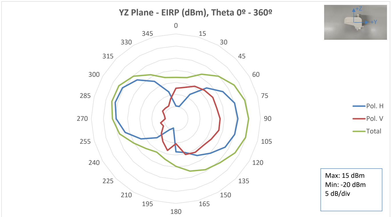
Fig. 12. YZ Plane EIRP, Free Space, 868.3 MHz.
