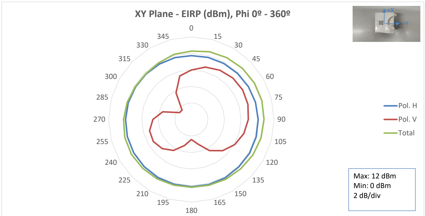
Fig. 13. XY Plane EIRP, Free Space, 869.525 MHz.
