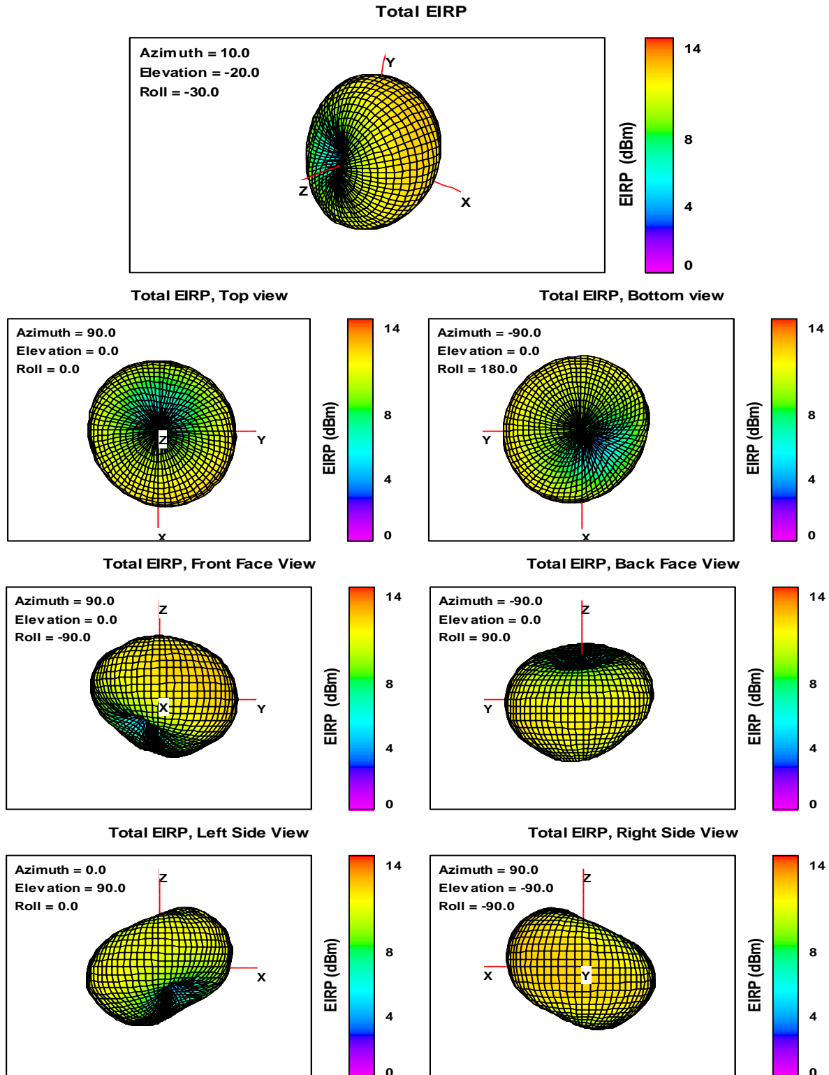
Fig. 21. Total EIRP, Free Space, 865.1 MHz.
