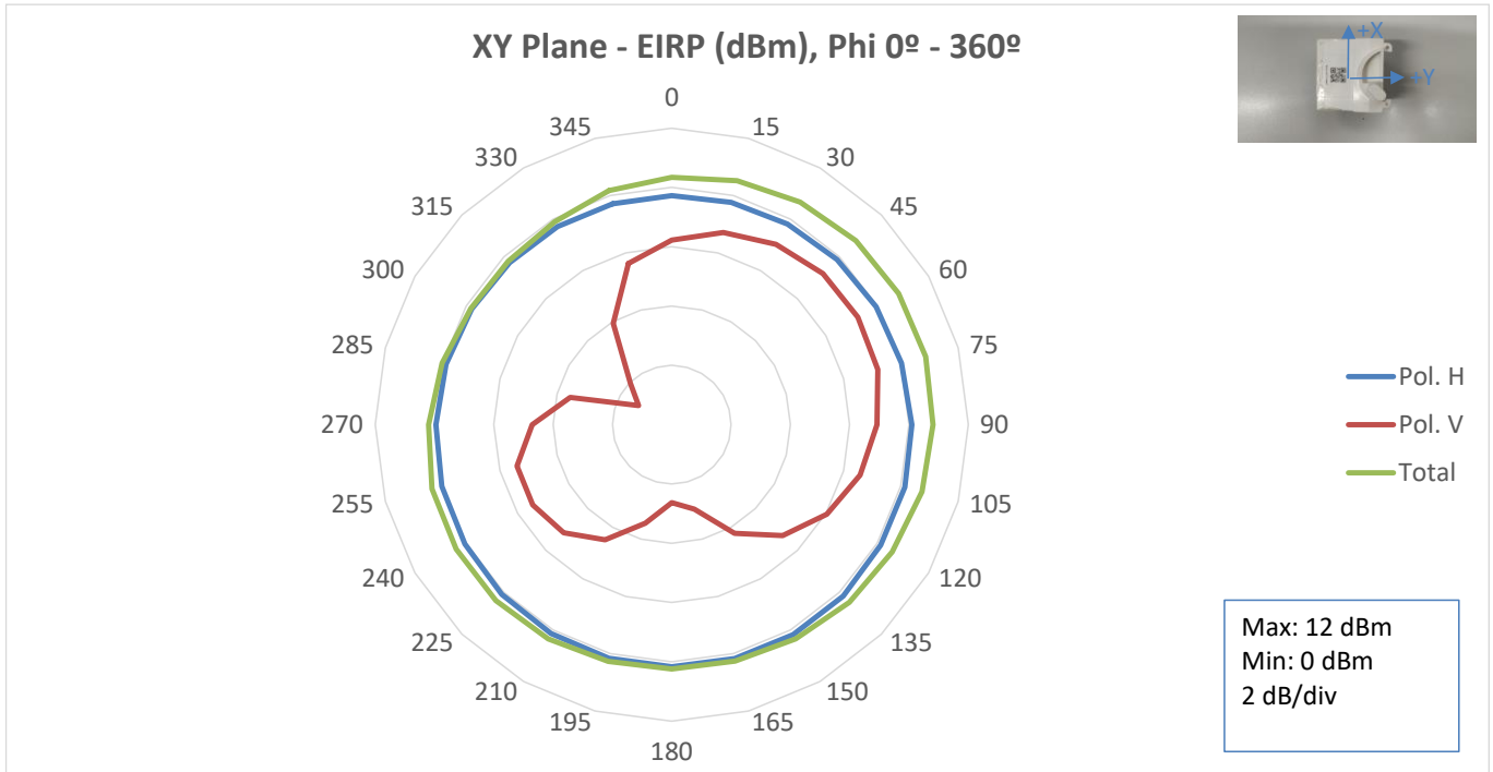
Fig. 10. XY Plane EIRP, Free Space, 868.3 MHz.
