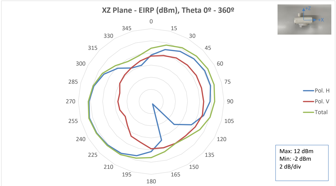
Fig. 8. XZ Plane EIRP, Free Space, 865.1 MHz.
