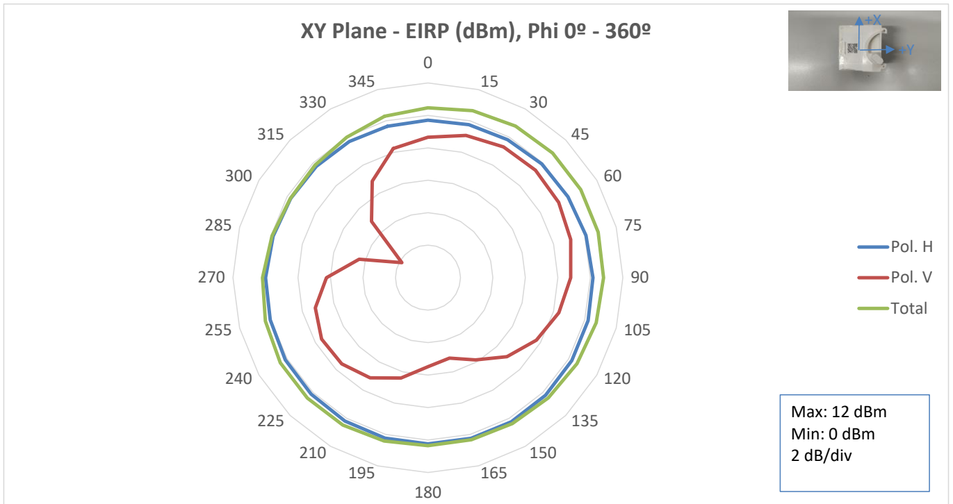
Fig. 7. XY Plane EIRP, Free Space, 865.1 MHz.
