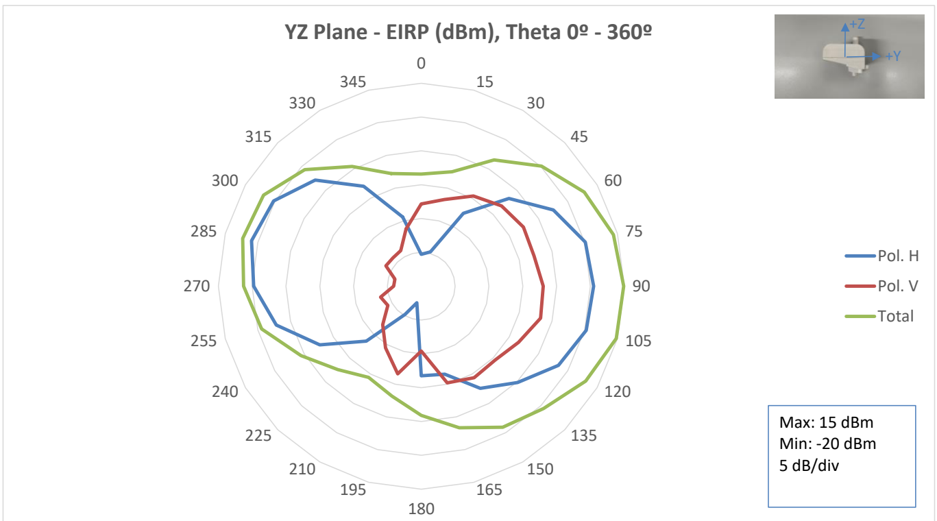
Fig. 15. YZ Plane EIRP, Free Space, 869.525 MHz.
