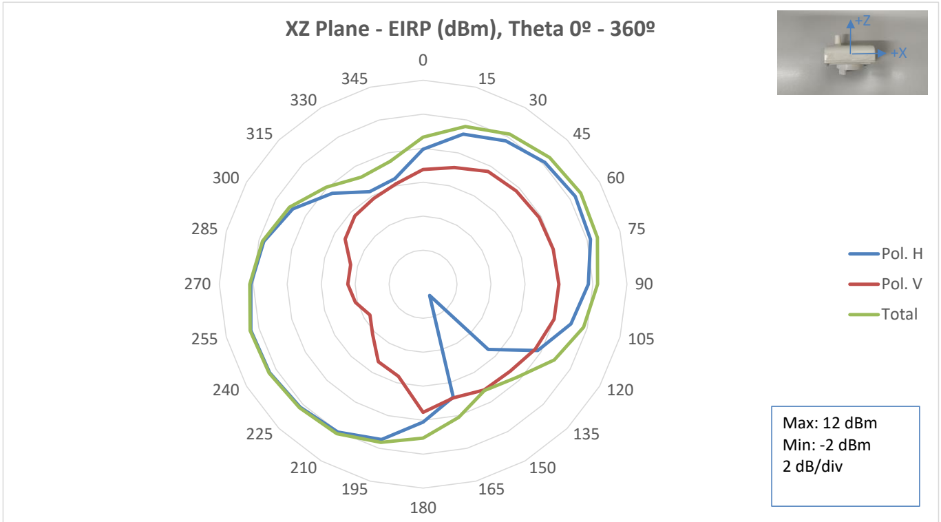
Fig. 14. XZ Plane EIRP, Free Space, 869.525 MHz.
