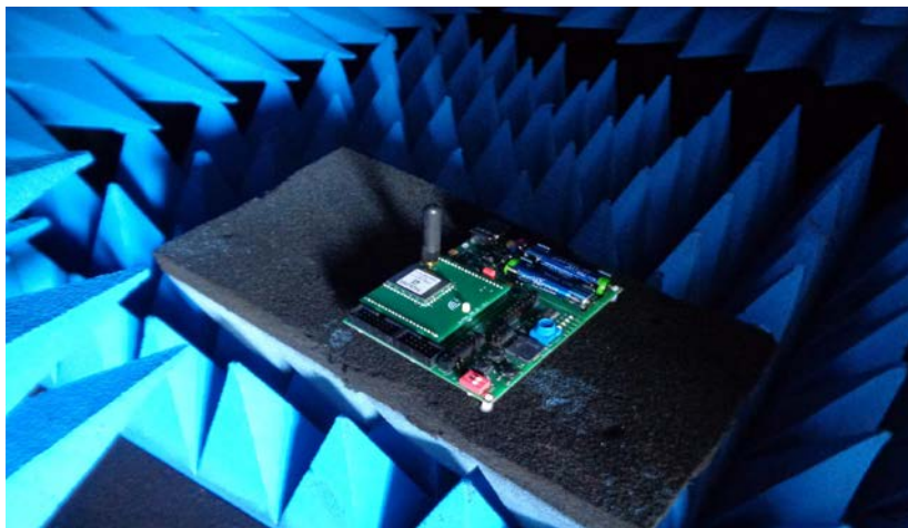
Figure 1 DUT Setup
