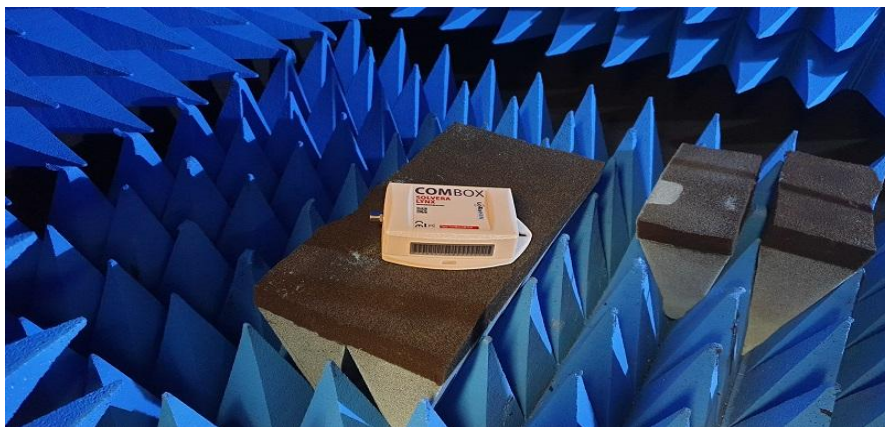
Figure 1 DUT Setup
