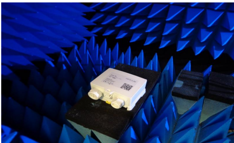
Figure 1 DUT Setup
