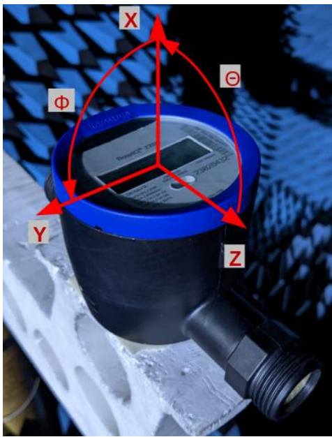
(a) Device under Test
