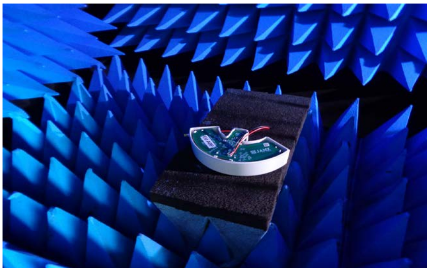
Figure 1 DUT Setup
