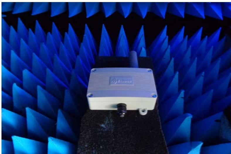
Figure 1 DUT Setup
