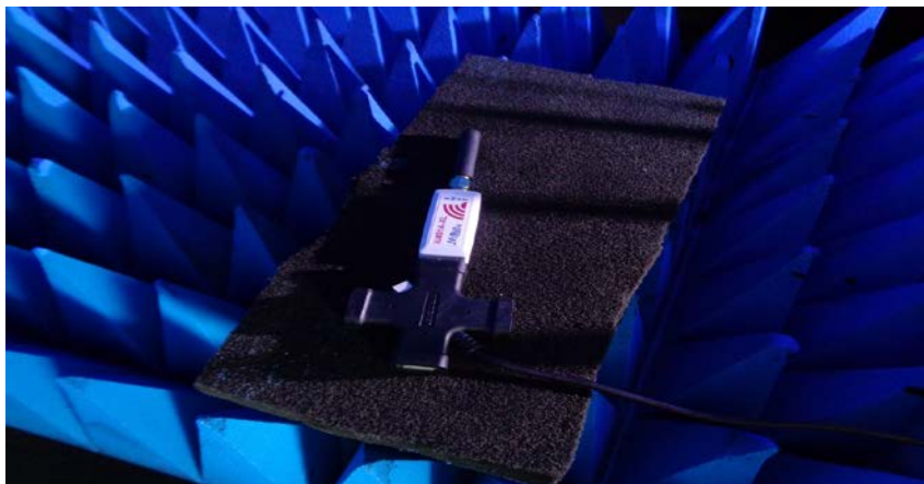
Figure 1 DUT Setup
