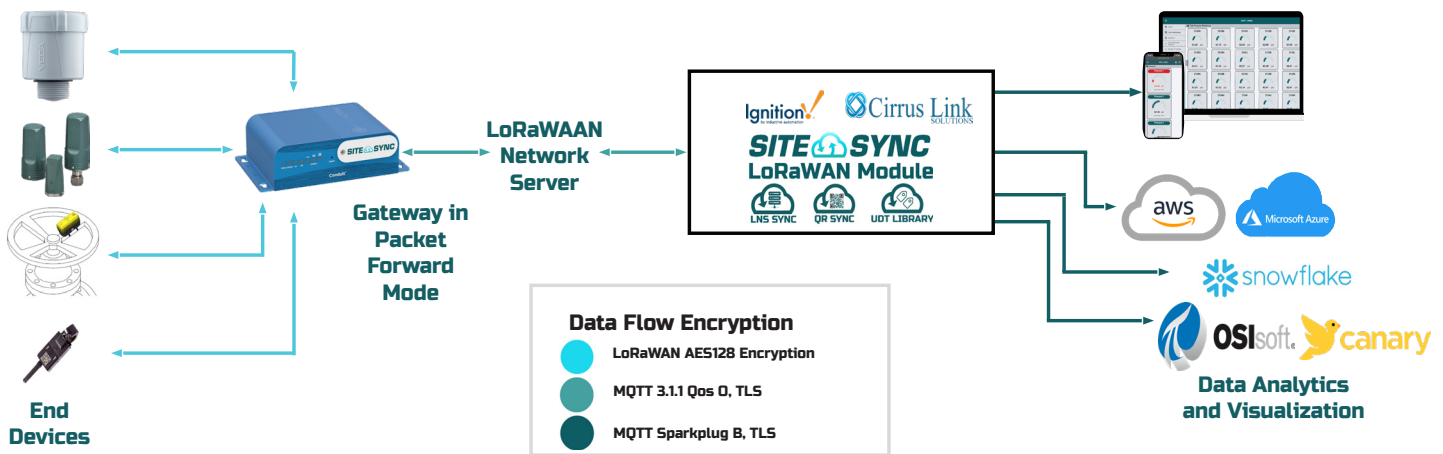
Figure 2. Displays the flow of data from End Devices to Data Analytics and Visualization platforms in a LoRaWAN Proof of Concept deployment.
