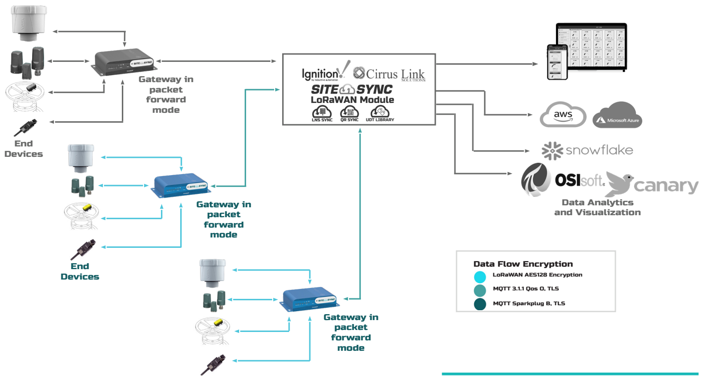
Figure 3. Displays a Sample Enterprise Wide LoRaWAN deployment utilizing many of the components already put in place during the Proof of Concept phase.
