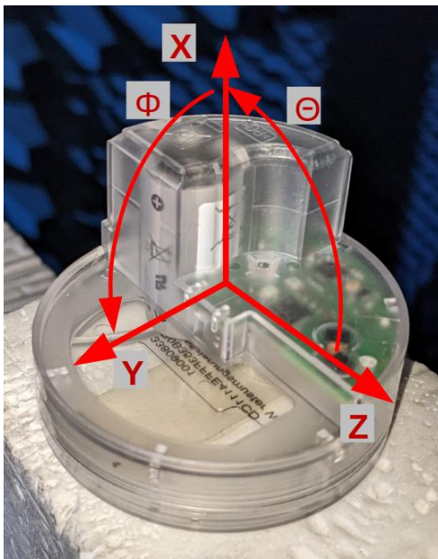
(a) Device under Test
